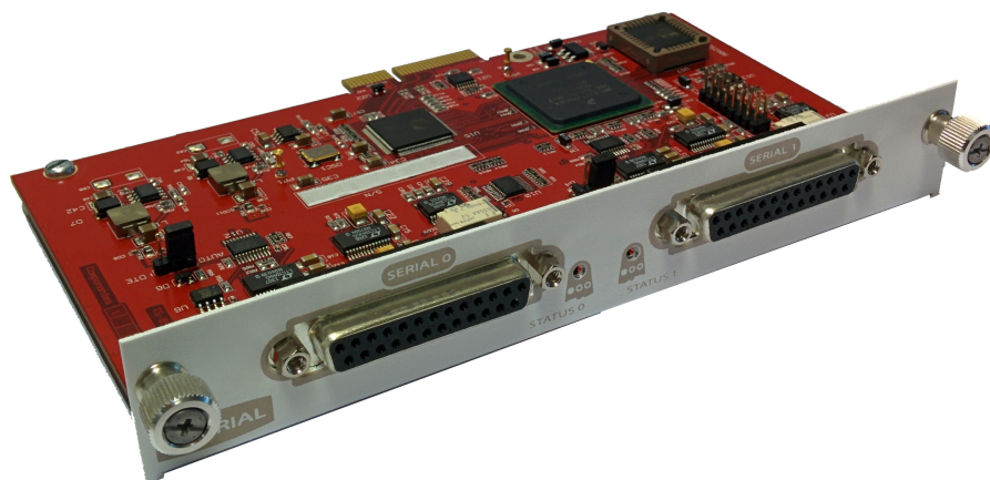
Fig. 1: TBC1-2SS card
